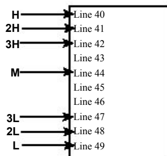
Figure 18.5 Cursor-positioning commands.
