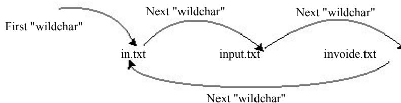
Figure 28.6 wildmode = full .
