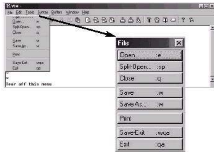
Figure 10.4 Tear-off menus.
