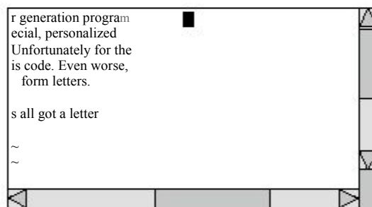
Figure 20.9 Horizontal scrolling.
