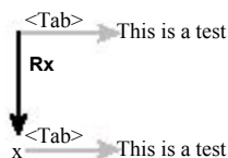
Figure 18.26 Virtual replacement.
