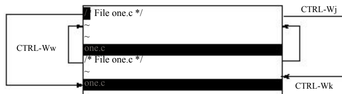
Figure 5.2 Window navigation.
