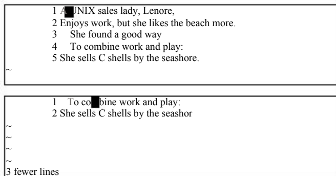
Figure 25.1 :1,3 delete.
