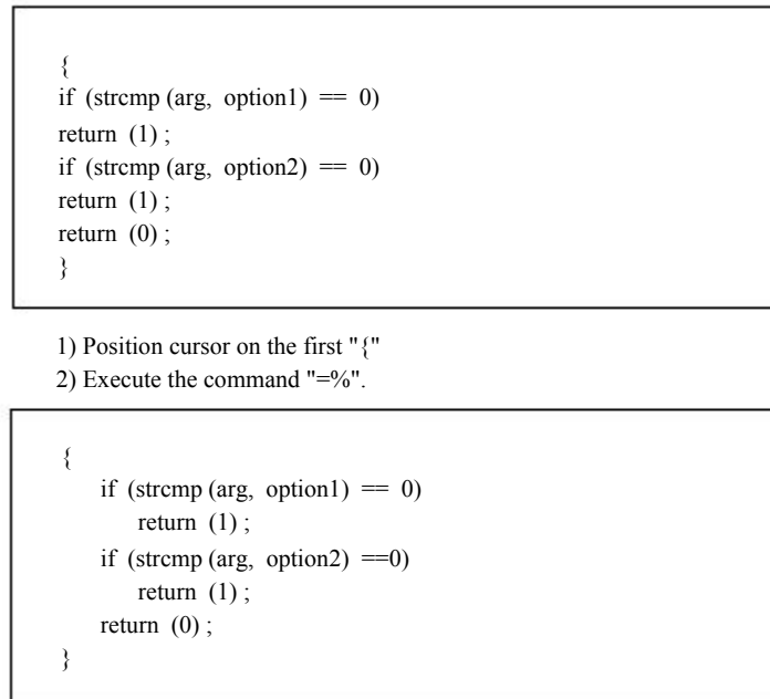
Figure 7.5 The = command.
