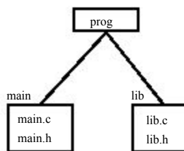
Figure 23.16 File layout.
