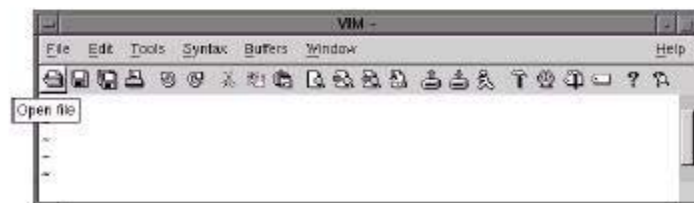
Figure 26.12 ToolTip.
