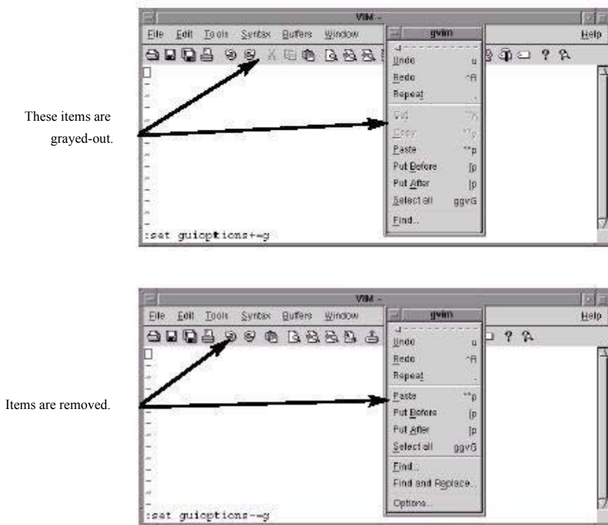
Figure 26.4 g option.
