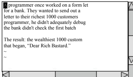
Figure 20.8 Horizontal scrollbar.
