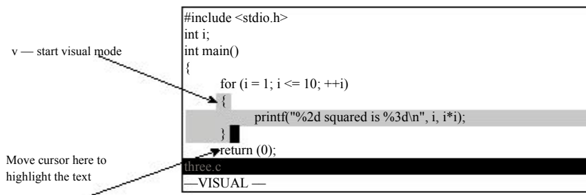
Figure 6.1 Visual mode.
