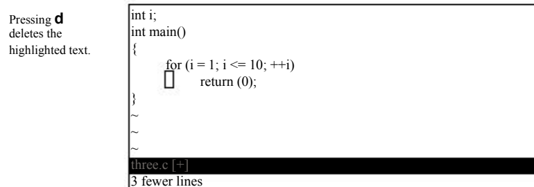
Figure 6.2 Visual delete.
