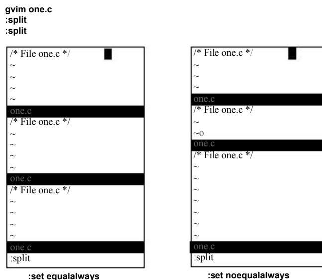
Figure 21.11 'equalways' option.
