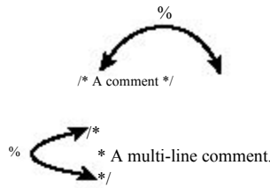
Figure 7.12 % and comments.
