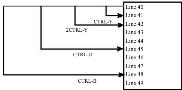
Figure 18.10 Scrolling commands.
